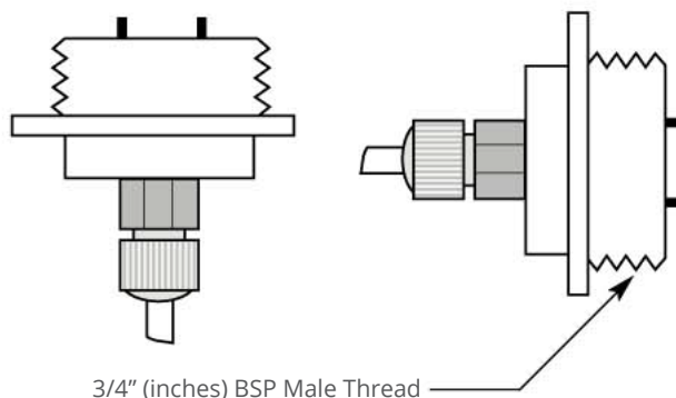
3/4" (inches) BSP Male Thread
